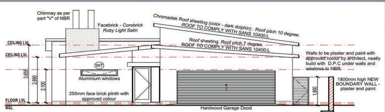
NORTH ELEVATION
